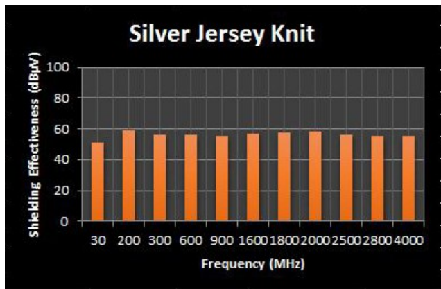
Shielding Effectiveness IEEE 299
