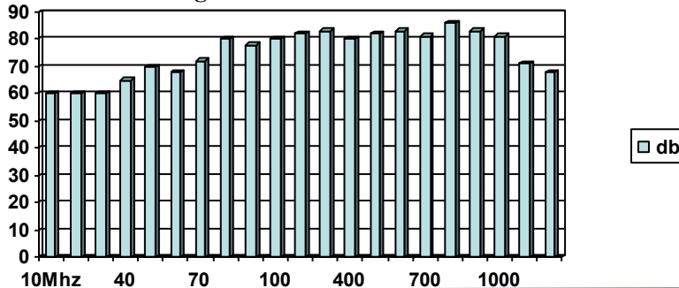
Shielding Effectiveness IEEE 299
