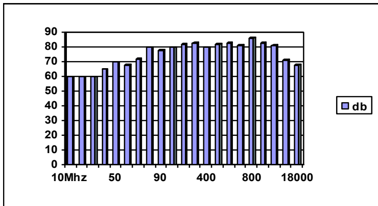
Shielding Effectiveness IEEE 299
