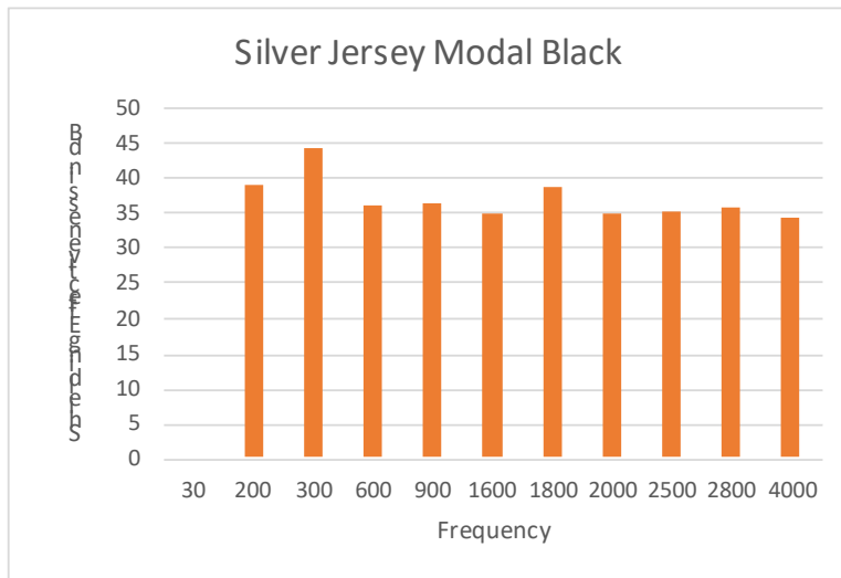
Shielding Effectiveness IEEE 299
